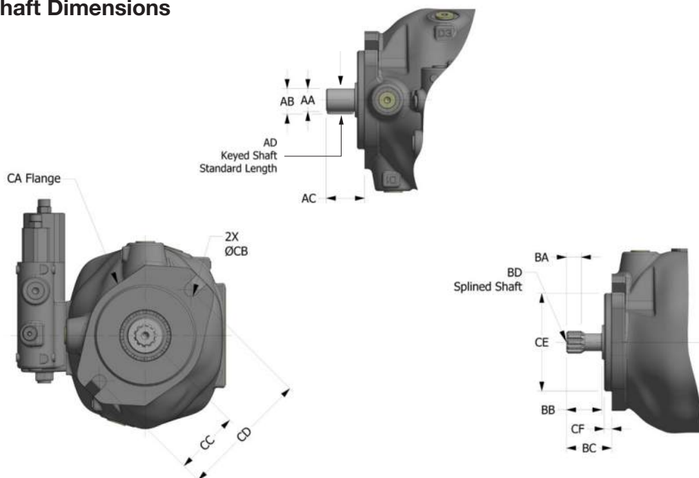
P1/PD-018 Mounting Flange &amp; Shaft Dimensions
