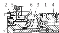
Model HED8OH-1XJ/...K14KW...
