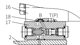
Illustration: directional valve opened
